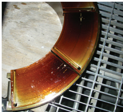
THRUST BEARING TILT PAD
