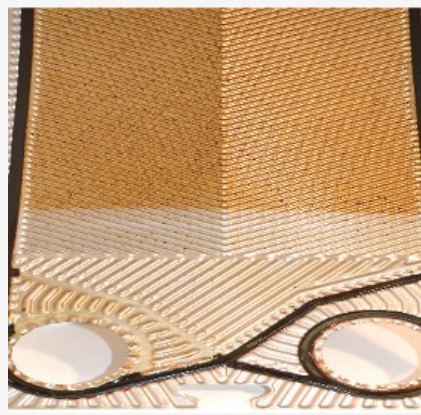
HEAT EXCHANGER COOLING PLATE
